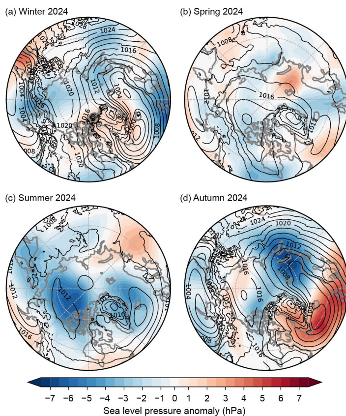
Fig. 5.7. Seasonal sea level pressure (SLP) anomalies (shading) and absolute values (isobars; both in hPa) in 2024 for (a) winter, (b) spring, (c) summer, and (d) autumn. SLP anomalies are shown relative to their 1991–2020 means. (Data source: ERA5 SLP data obtained from the Copernicus Climate Change Service.)
