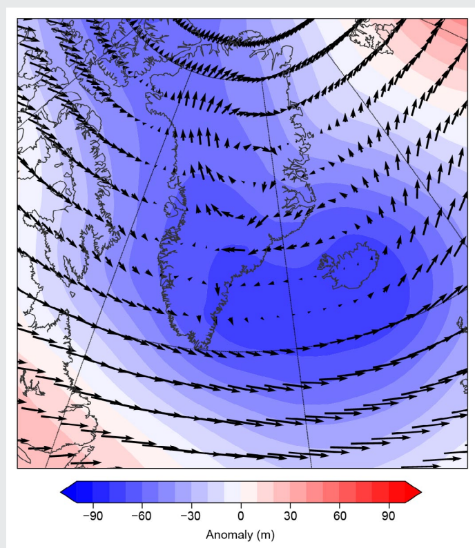
Fig. SB5.5. Jul–Aug 2024 ERA5 (Hersbach et al. 2020) wind vectors (arrows, \text{m s}^{-1} ) at 700 hPa and geopotential height anomalies (m) at that level, approximately 3000 m above sea level, indicate the prevailing pattern during mid-to-late melt season. The 2024 season was marked by suppressed melt that resulted from cold polar air flowing southward along the western ice sheet where most surface melting typically occurs.
