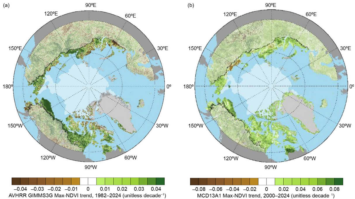
Fig. 5.33. Magnitude of the Maximum Normalized Difference Vegetation Index (MaxNDVI) trend calculated as the change decade -1 via ordinary least-squares regression for Arctic tundra (solid colors) and boreal forest (muted colors) north of 60° latitude during (a) 1982–2024 based on the Advanced Very High-Resolution Radiometer (AVHRR) Global Inventory Modeling and Mapping Studies third generation (GIMMS-3g+) dataset, and (b) 2000–24 based on the Moderate Resolution Imaging Spectroradiometer (MODIS) MCD13A1 dataset. The circumpolar tree line is indicated by black lines, and the 2024 minimum sea ice extent is indicated by light shading in each panel.
