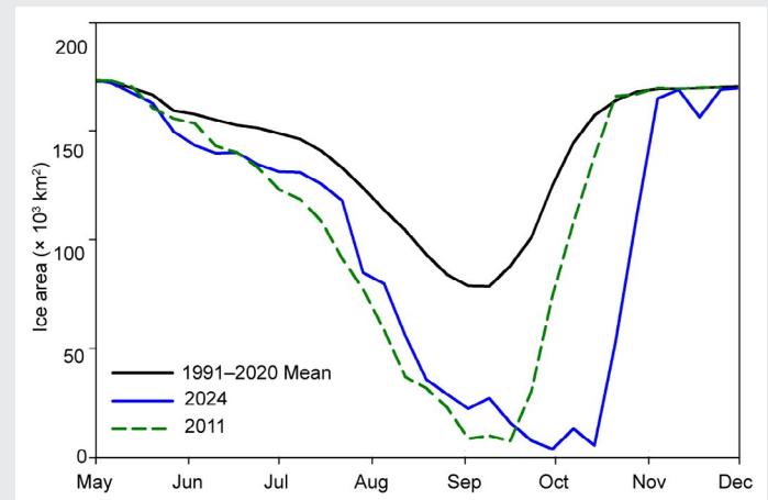
Fig. SB5.3. Time series of total sea ice area ( \times 10^3 \text{ km}^2 ) within the Northwest Passage northern route for 2024 (solid blue line), 2011 (dashed green line), and the 1991–2020 mean (solid black line). (Data source: Canadian Ice Service.)
