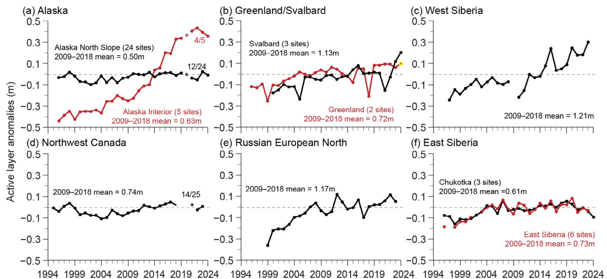
Fig. 5.29. Average annual active-layer thickness (ALT) anomalies (m), relative to the 2009–18 mean, for six Arctic regions observed by the Circumpolar Active Layer Monitoring program. Positive and negative anomalies indicate thicker or thinner ALT than the 10-year reference, respectively. Numbers of sites vary by region because only sites with >20 years of continuous thaw depth observations from the end of the thaw season are included. Asterisks represent atypical observations, for example, due to pandemic-related restrictions (fraction of sites for these years are provided on graph). Canadian ALT is derived from thaw tubes that record the maximum thaw depth over the previous year. Since Canadian sites were not visited in 2020 and 2021, the maximum thaw depth recorded during the 2022 visit could have occurred during any summer between 2019 and 2021, although the data point is plotted in 2021. Site-specific data and metadata are available at https://www2.gwu.edu/~calm/ .
