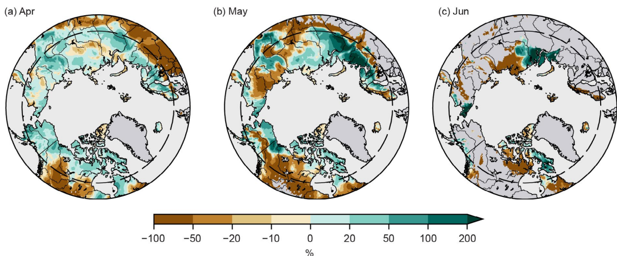
Fig. 5.26. Snow water equivalent (SWE) anomalies (% difference from the 1991–2020 baseline) in 2024 for (a) Apr, (b) May, and (c) Jun. Brown (green) indicates lower (higher) snow amounts than average. Latitude 60°N is marked by the gray dashed circle. (Data source: selection of four SWE products from Snow Climate Change Initiative [CCI; Luoju et al. 2022]; MERRA-2 [GMAO 2015]; ERA5-Land [Muñoz Sabater 2019]; and Crocus [Decharme et al. 2024].)
