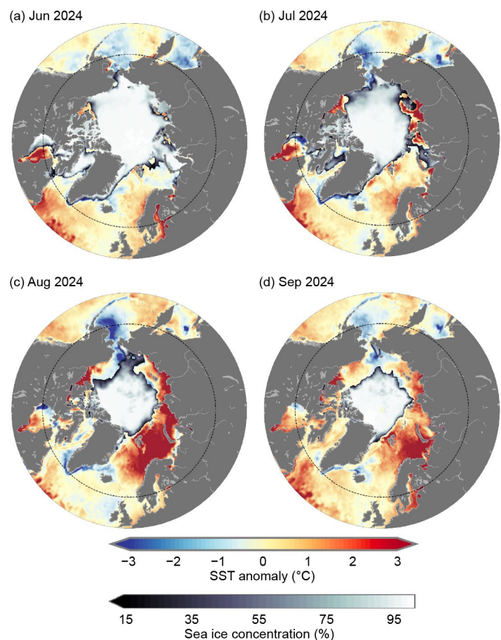
Fig. 5.12. Sea surface temperature (SST) anomalies (°C) for (a) Jun 2024, (b) Jul 2024, (c) Aug 2024, and (d) Sep 2024 relative to the 1991–2020 mean for the respective months. The mean sea ice concentration for the corresponding month is also shown. While sea ice extent is lowest in Sep, SSTs cool in the latter part of the month. The dashed circle indicates the latitudinal bound of the maps in Fig. 5.11. See Fig. 5.11 caption for sea ice dataset information.
